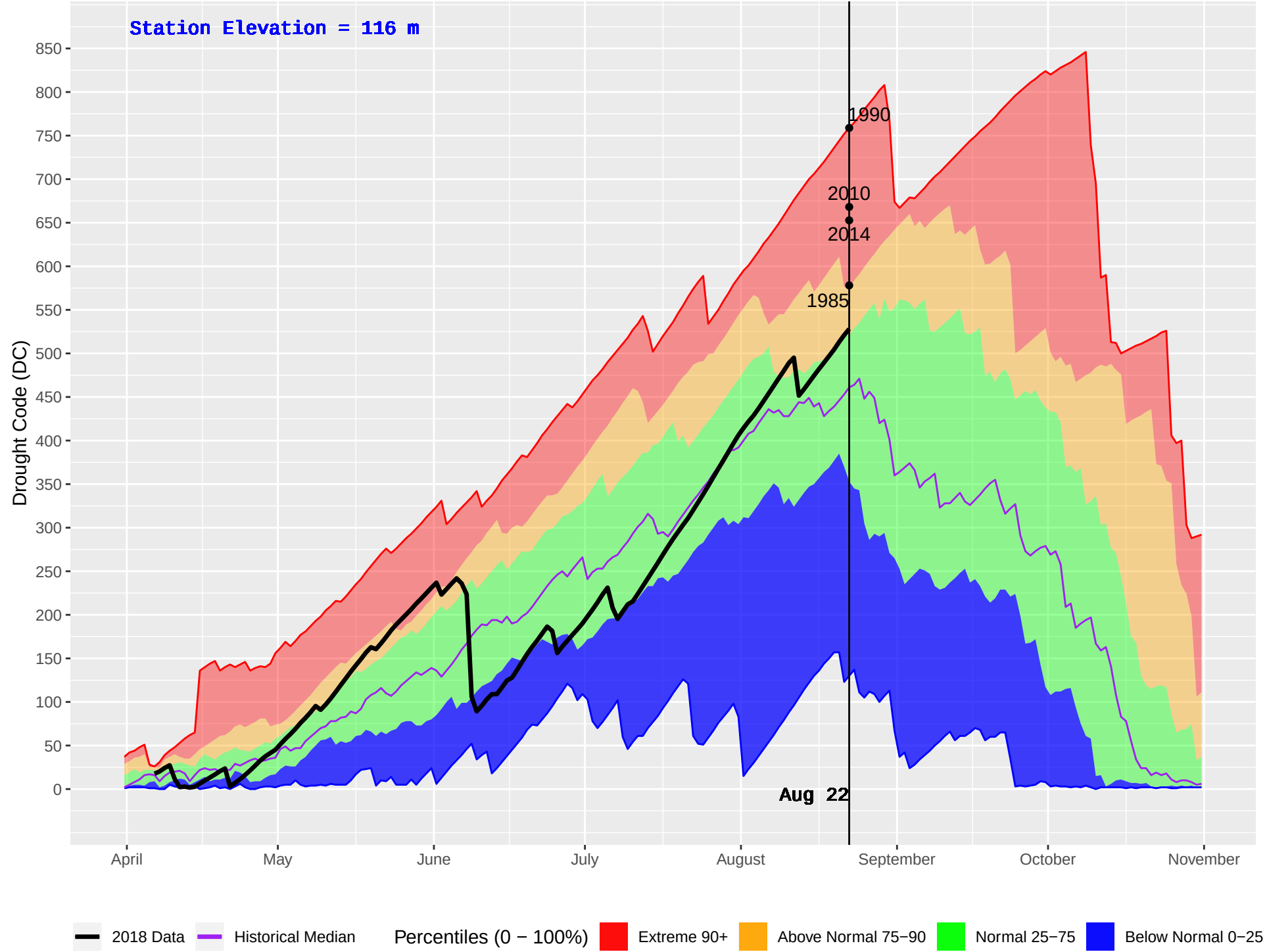
SCAR CREEK (82) : Historical (1982–2016) and Current (2018) Daily Drought Code (DC)
