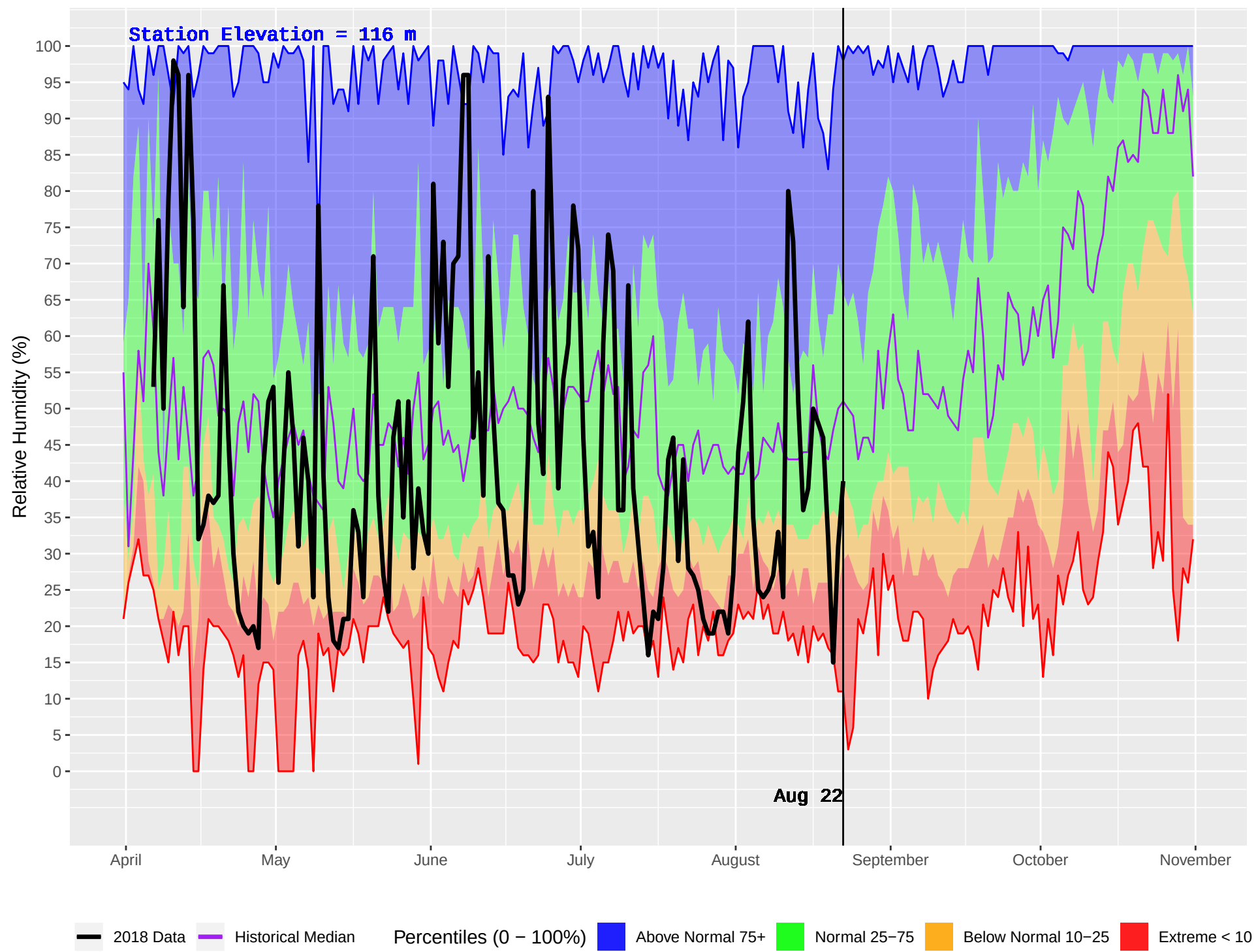
SCAR CREEK (82) : Historical (1982–2016) and Current (2018) Daily Relative Humidity
