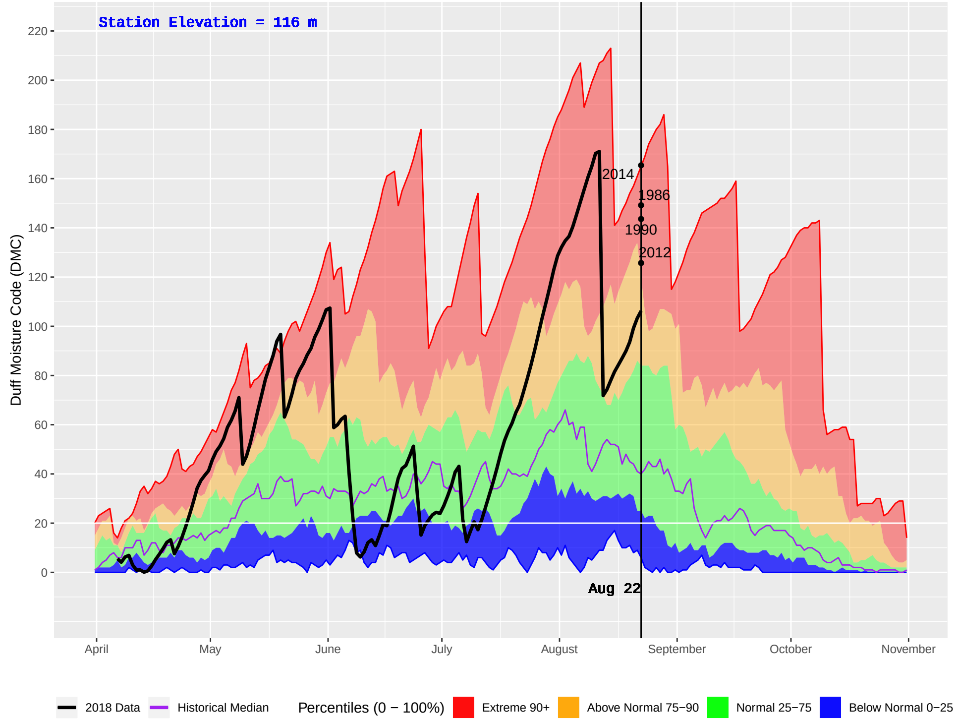
SCAR CREEK (82) : Historical (1982–2016) and Current (2018) Daily Duff Moisture Code (DMC)
